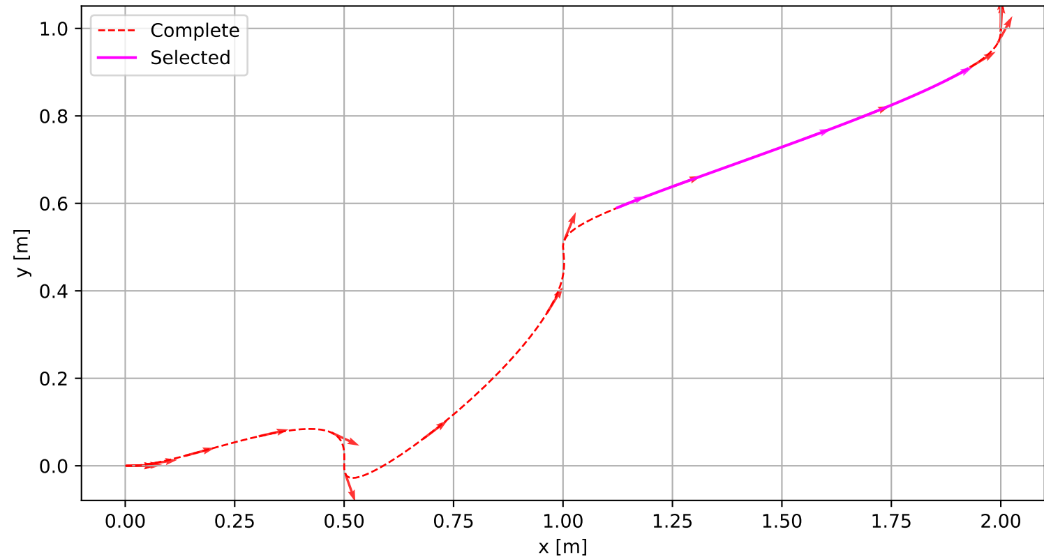
Trajectory Comparison
